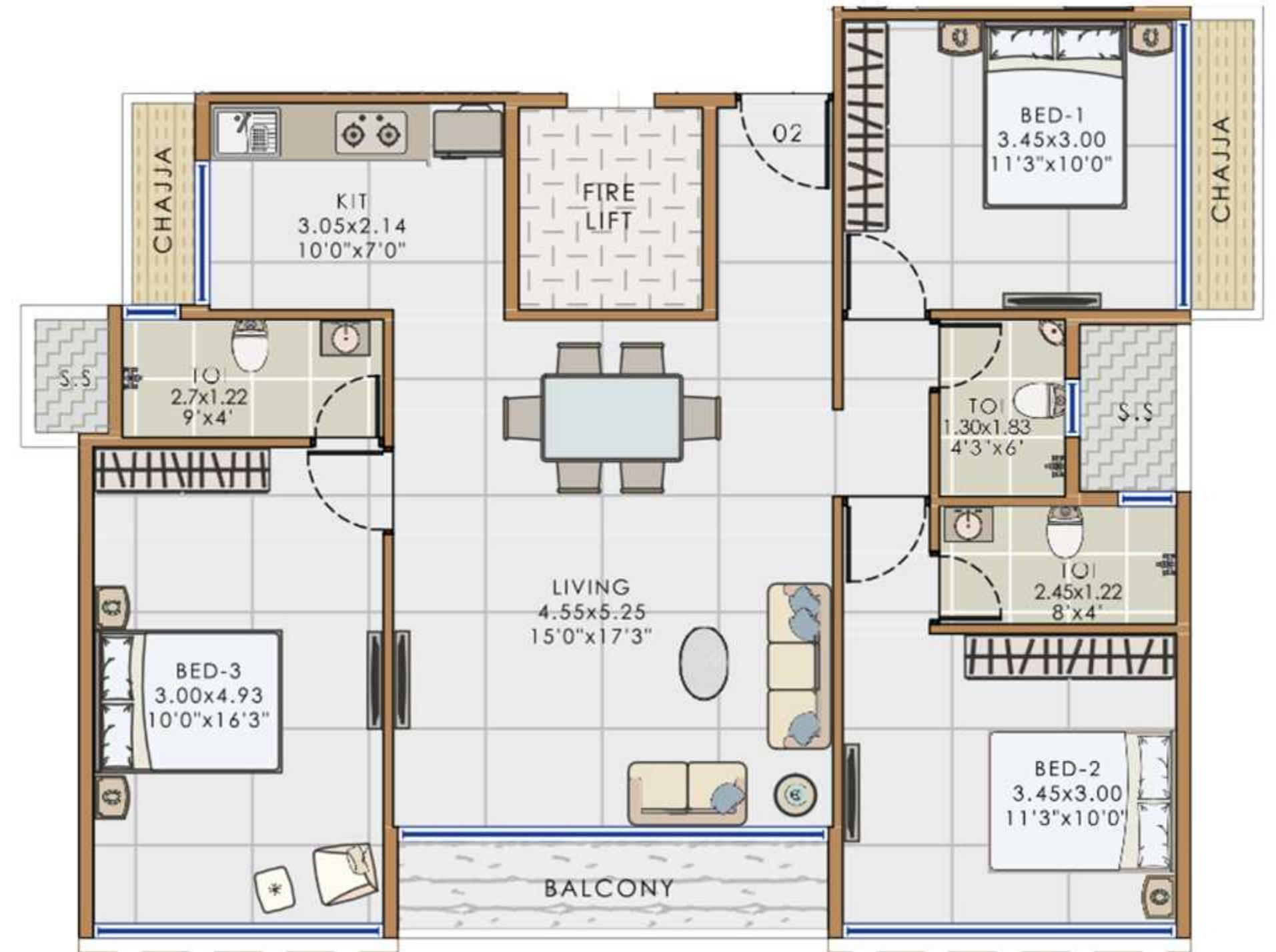
1ST TO 5 TH FLOOR PLAN 3 BHK FLOOR PLAN
